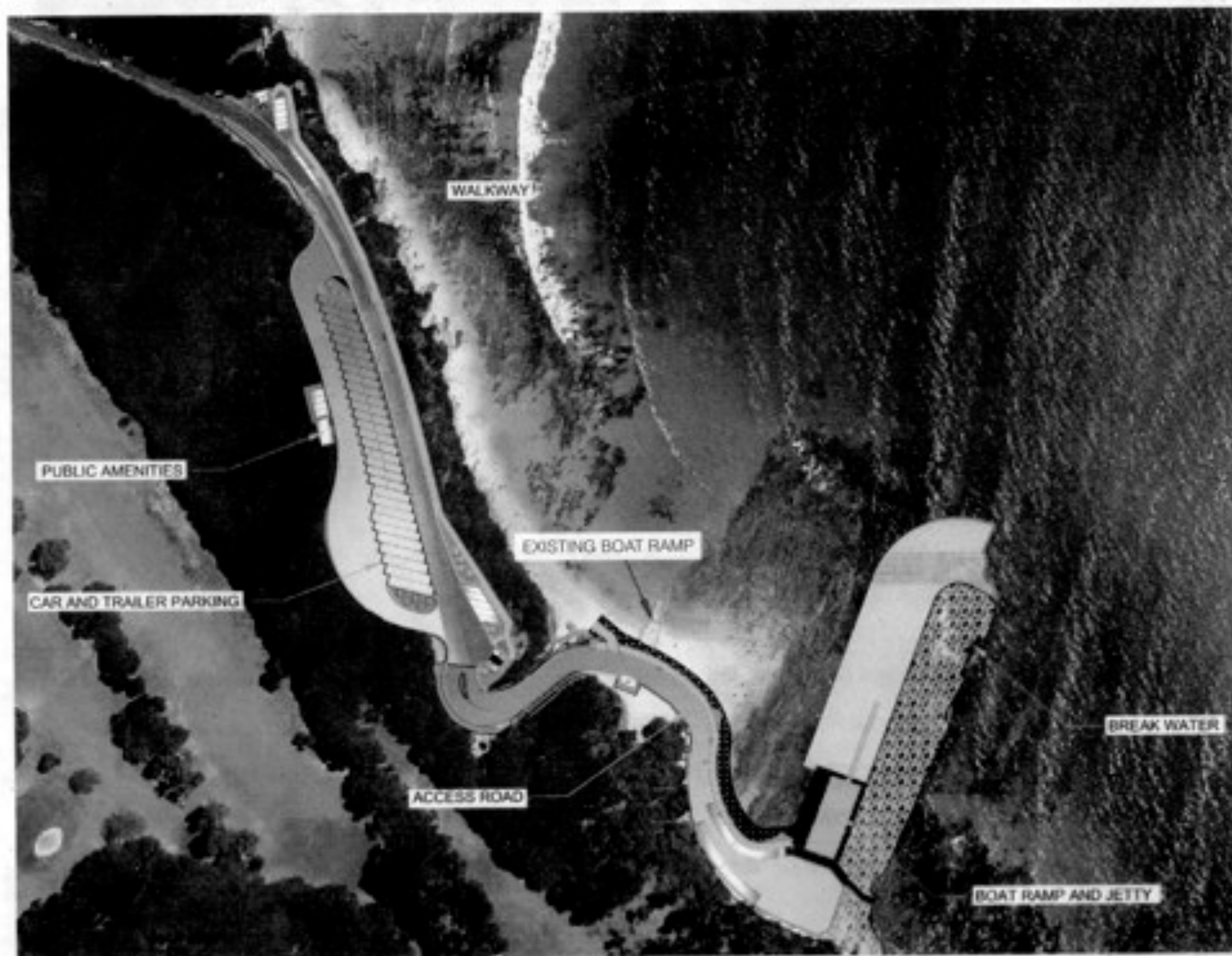
The new boat ramp and breakwater will dramatically improve the launching of recreational and commercial vessels and vehicle parking facilities.
